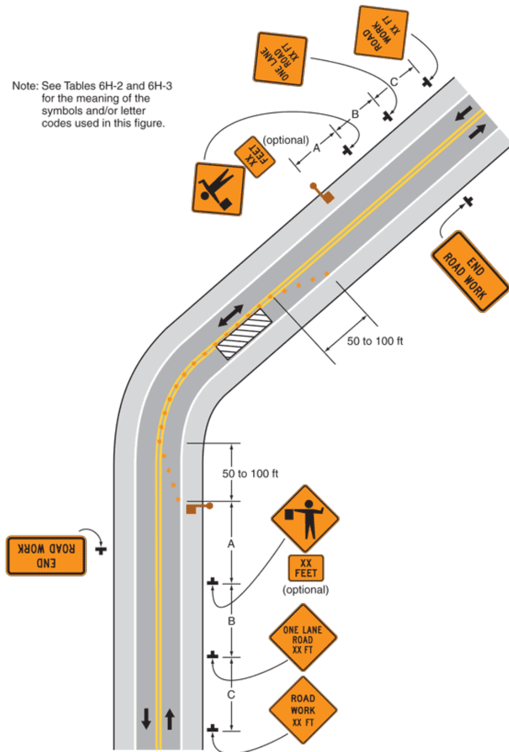
Typical Application 10
